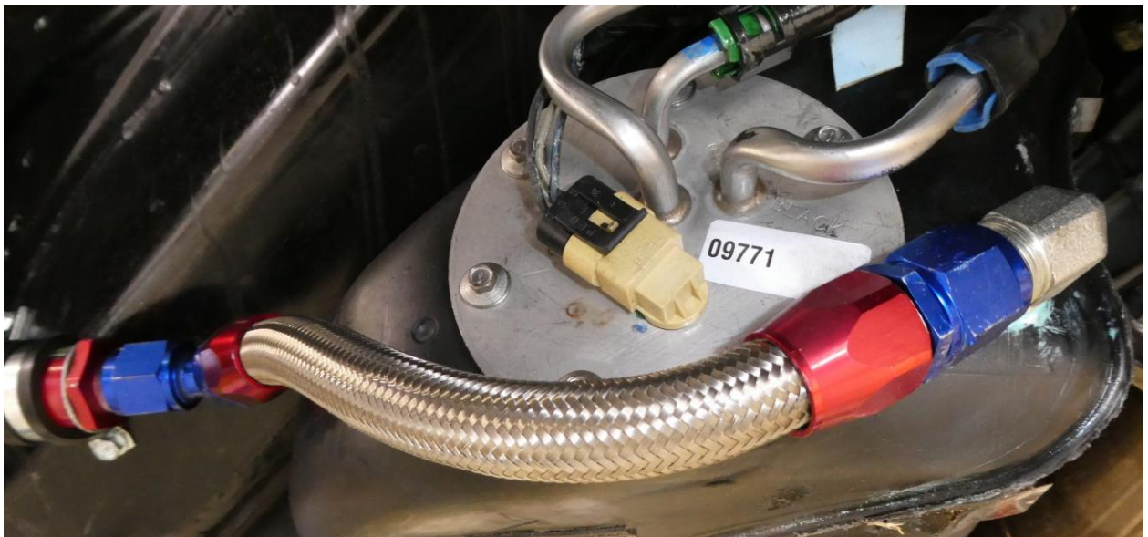
FUEL LINE FROM TANK FITTING TO PUMP
